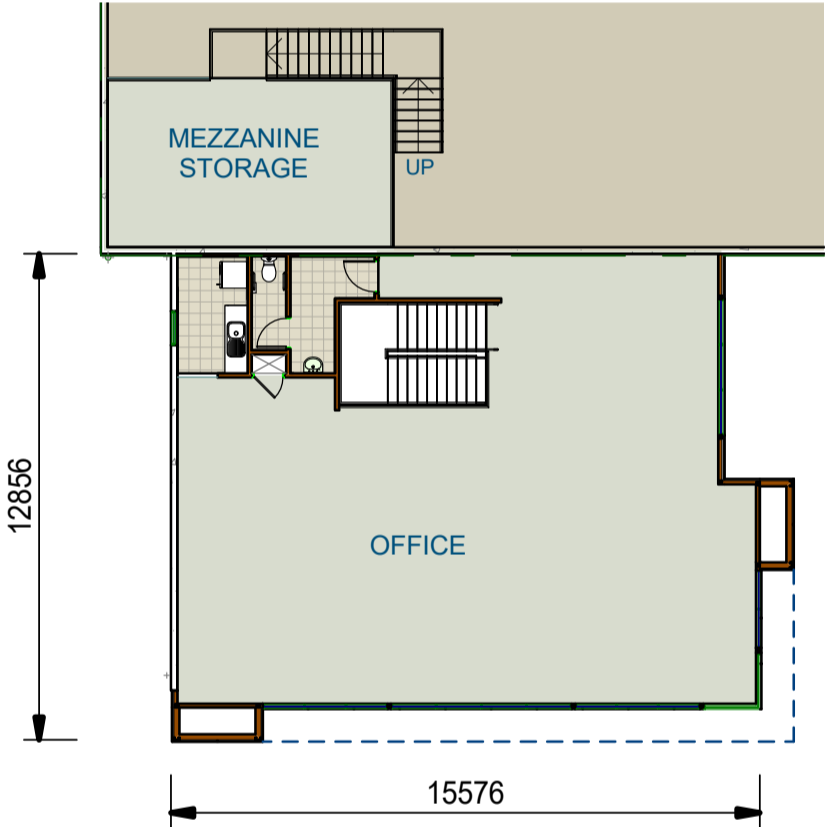
LEVEL 1 OFFICE PLAN NTS
